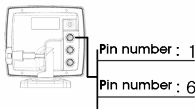
Output (2) NMEA 0183
