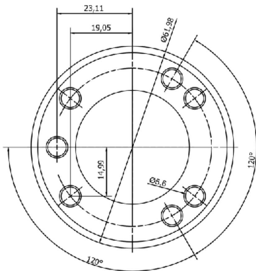
RAM MOUNTING - METRIC
