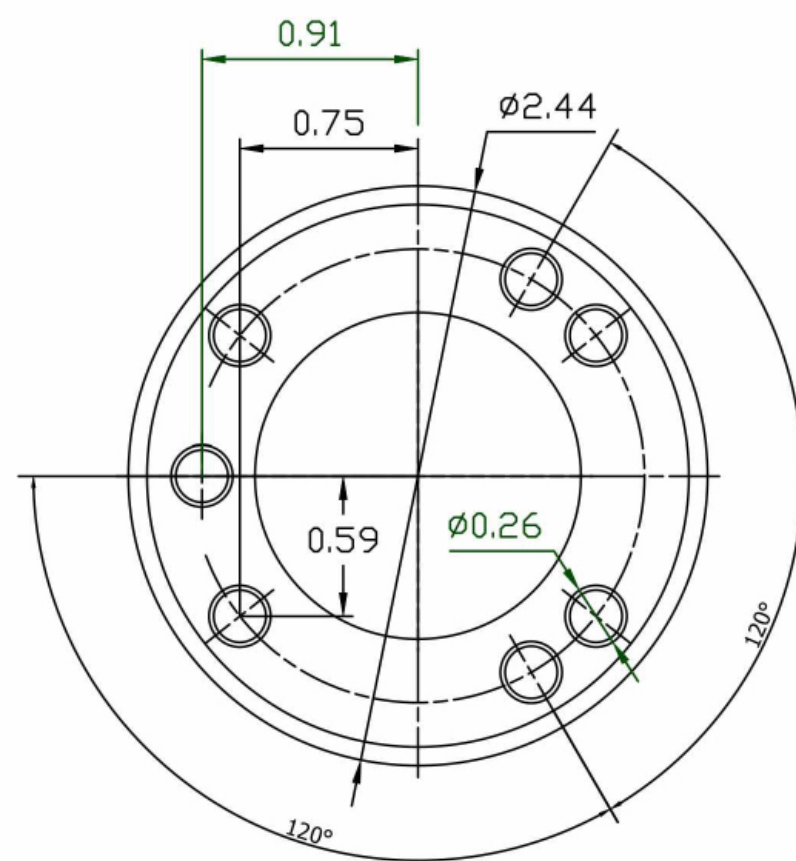
RAM MOUNTING - INCHES
